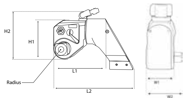
Square Drive hydraulic torque wrench dimensions
